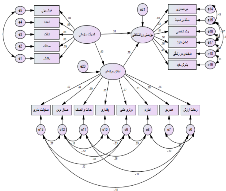
Figure 2. Research model with standard path coefficients
